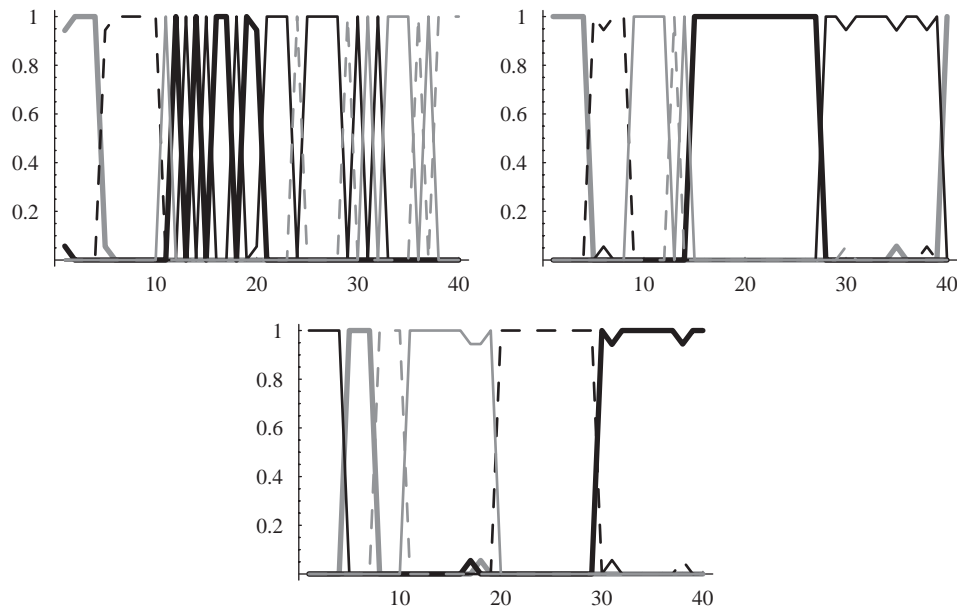
Fig. 10. Discrimination–similarity game of a reinforcement learner with a non-constant k_{\text{sim}} . Parameters are n = 40 , m = 6 , L = 15 , k_{\text{sim}} varies between 2 for chips 1–10 and 6 for chips 11–40. The last frame is taken after about 10^7 runs.
